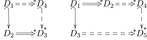
Fig. 1. Lift and Project properties.
