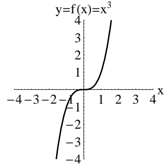
Cubing Function
