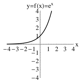
Exponential Function
