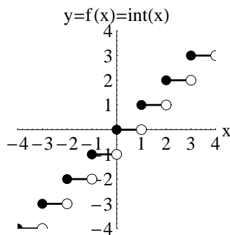
Greatest Integer Function
