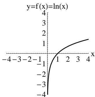
Natural Logarithmic Function
