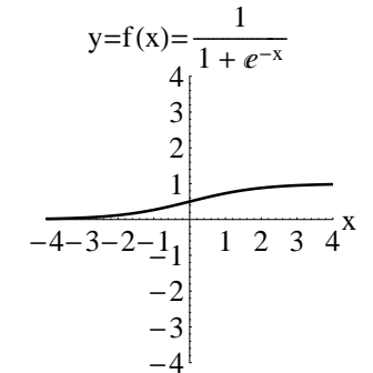
Logistic Function
