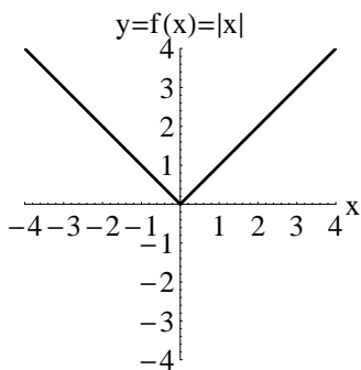
Absolute Value Function
