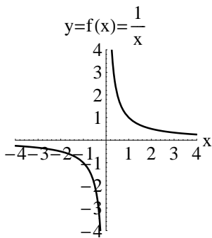
Inverse Function
