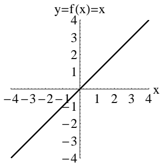
Identity Function
