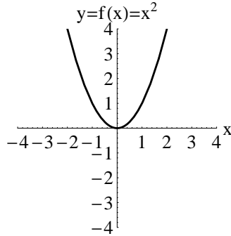
Squaring Function
