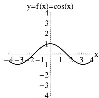
Cosine Function
