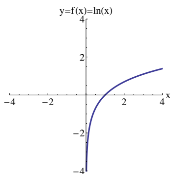
Natural Logarithmic Function
