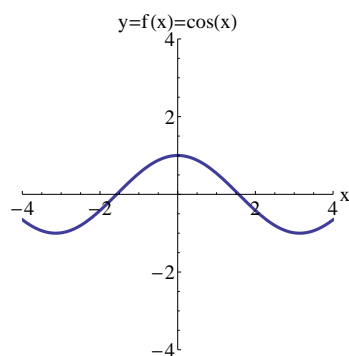
Cosine Function
