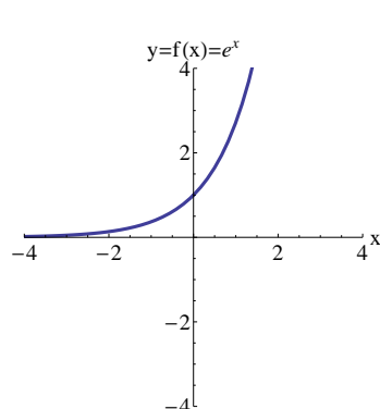
Exponential Function
