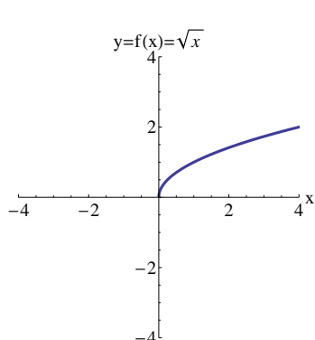
Square Root Function
