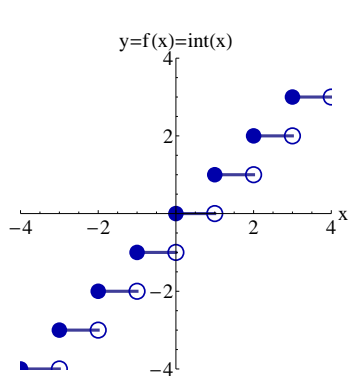
Greatest Integer Function
