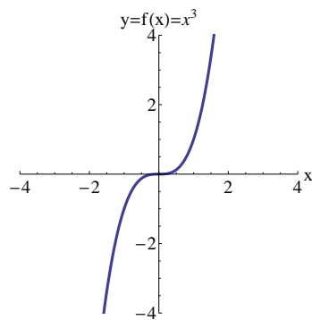
Cubing Function
