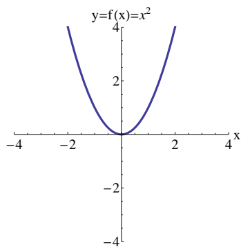
Squaring Function
