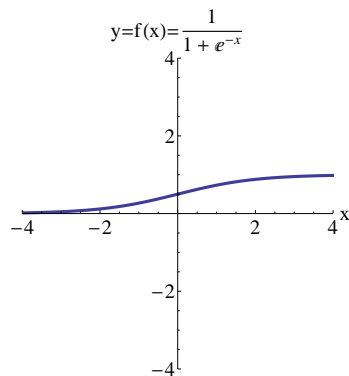
Logistic Function
