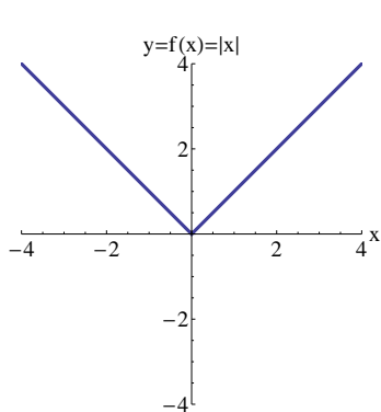
Absolute Value Function
