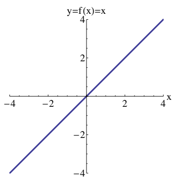
Identity Function
